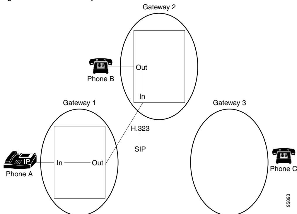
Figure 1-37 Three Gateways: Cisco CME IP Phone XOR Before Transfer
