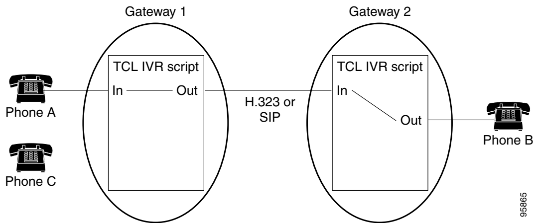
Figure 1-9 Two Gateways (XOR/XTO & XEE): Analog XOR Before Transfer
